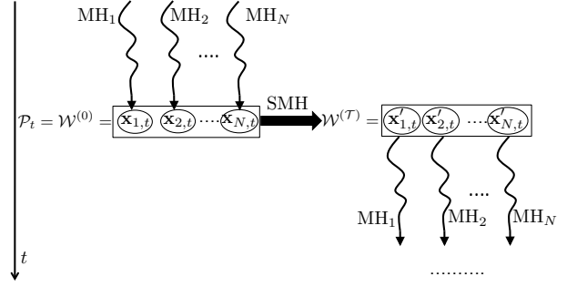
Fig. 1. Sketch of the O-MCMC technique.
